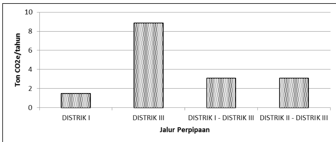
Gambar 7 Beban emisi pipeline blowdowns
