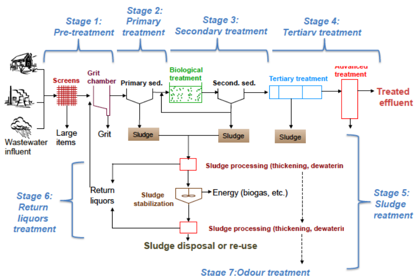
Fig 1. General schematic representation of a WWTW with the various stages [2]
