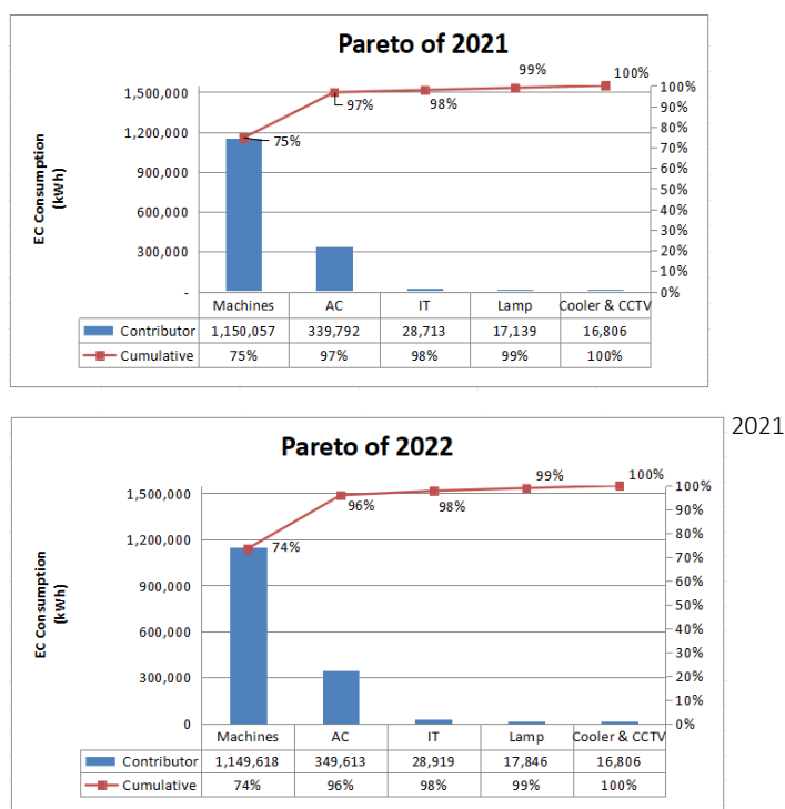
Figure 3 Pareto Electricity Consumption 2022
