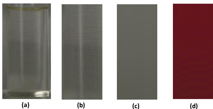
Fig. 1. Digital mage processing using OpenCV on Pt-Co Sample on a light background. (a) Original image (120x240 pixels), (b) ROI (175x75 pixels), (c) Normalized box filter application (200x200 pixels), (d) HSV color space of sample image
