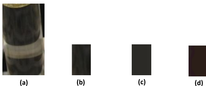
Fig 2. Digital mage processing using OpenCV on Pt-Co Sample on Pt-Co Sample on dark background. (a) Original image (175x75 pixels), (b) ROI (52x32 pixels), (c) Normalized box filter application (200x200 pixels), (d) HSV color space of sample image
