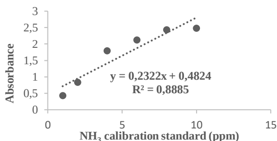
Fig. 7. The Plot Graph of Linear Regression Result of \text{NH}_3 phenate Absorbance Values and its Predicted Concentration (ppm)
