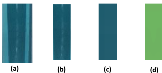
Fig. 5. Digital mage processing using OpenCV on \text{NH}_3 Phenate Sample on a (a) Original image (50x100 pixels), (b) ROI (95x30 pixels), (c) Normalized box filter application (100x100 pixels), (d) HSV color space of sample image
