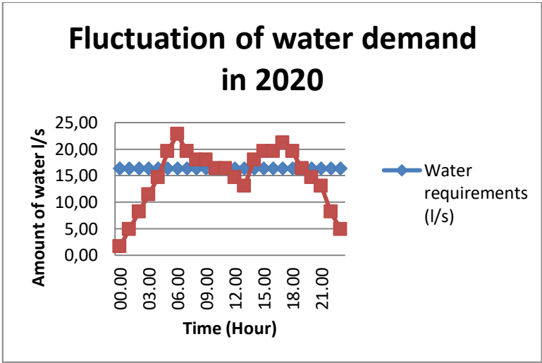
Fig.6 Fluctuation of water demand in 2020
