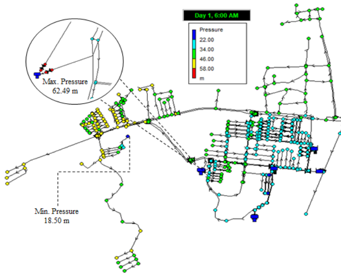
Fig. 9. The simulation results of the pressure on each node during peak hours
