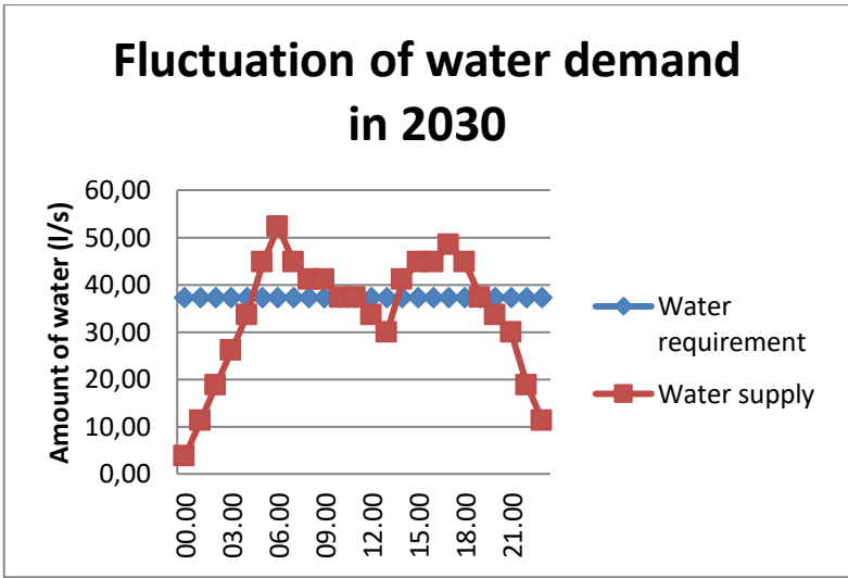
Fig. 7. Fluctuation of water demand in 2030
