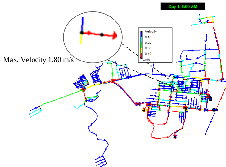
Fig. 10. The simulation results of velocity in each pipe during peak hours
