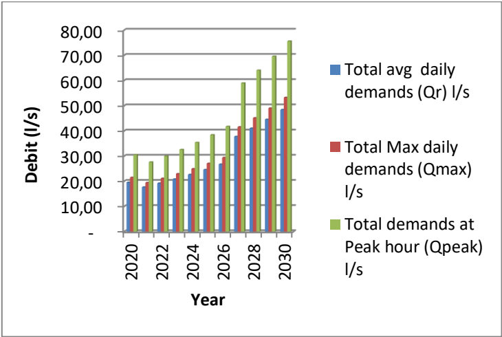
Fig. 5. Projection of clean water demand from 2020-2030
