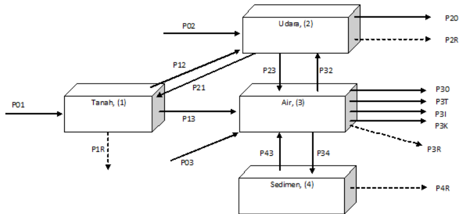
Gambar 1. Diagram konseptual model fugasitas di Waduk Saguling
