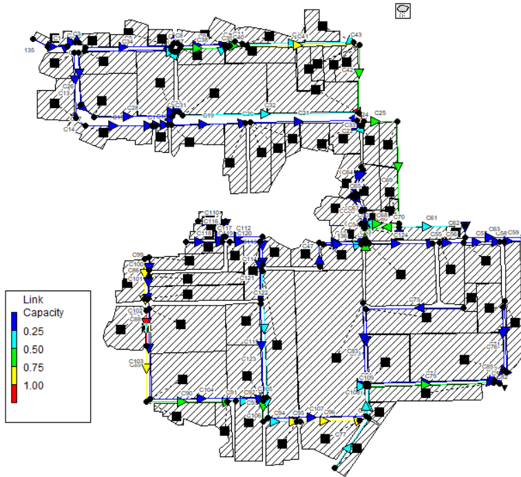
Fig.7. Simulation of drainage system models and study area flow patterns in the first hour.
