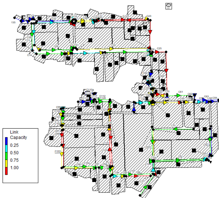
Fig.8. The second-hour simulation of drainage network models and research region flow patterns.
