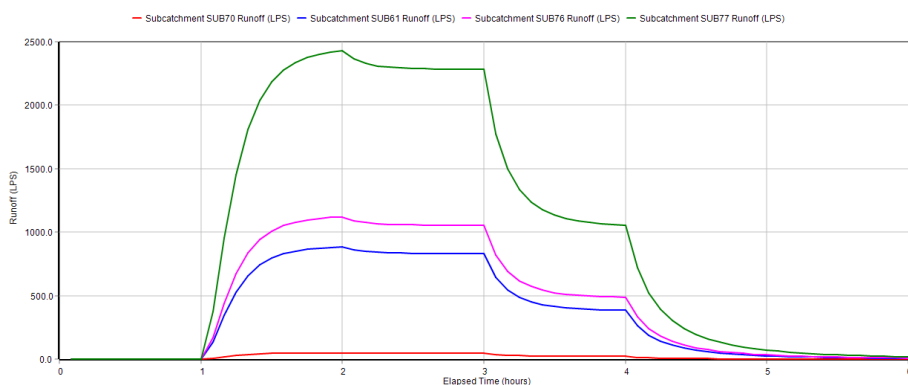
Fig.9. The graphic of runoff on the elapsed time.
