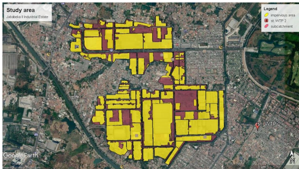
Fig.6. The impervious area condition in subcatchment. (yellow color is impermeable sub-area and purple color is subcatchment area)
