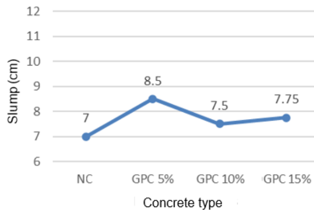
Fig. 8 Slump height of the glass powder concrete and normal concrete
