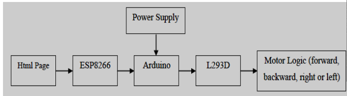
Figure 9. Block Diagram of System's Operation
